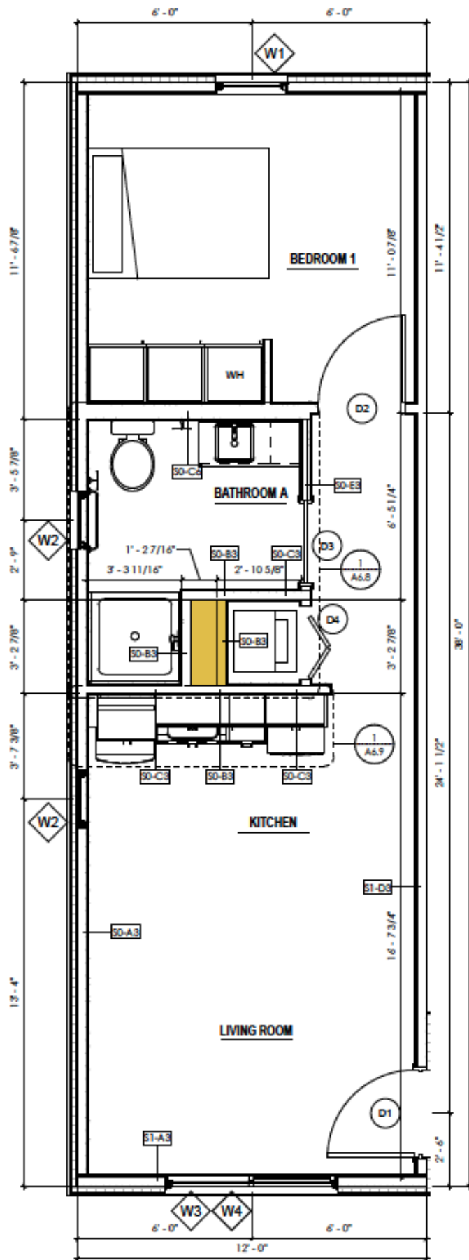
UNIT 1 ENLARGED PLAN 3/8" = 1'-0"
