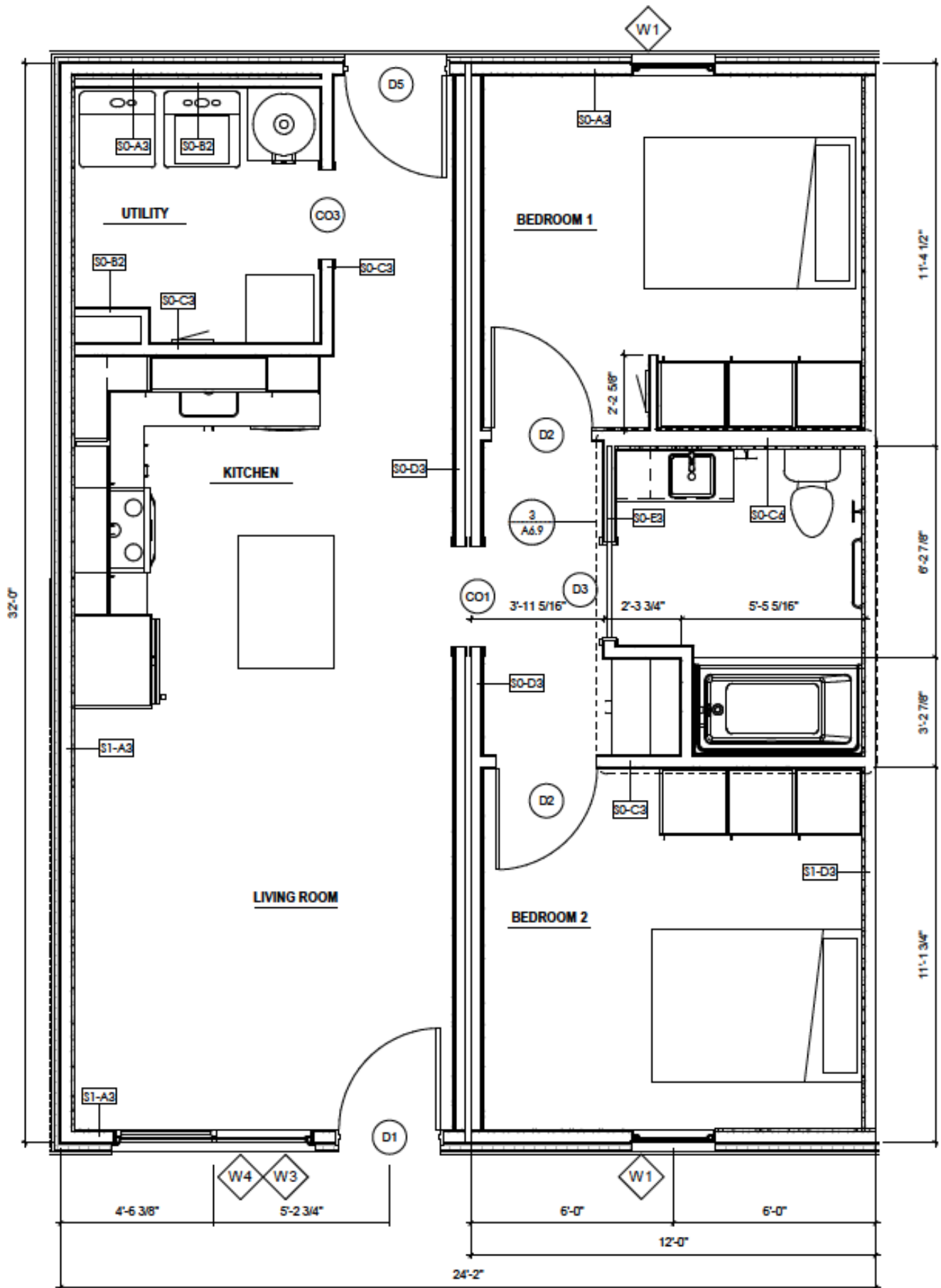
BUILDING 2, LEVEL 1, UNIT 1 FLOOR PLAN 3/8" = 1'-0"
