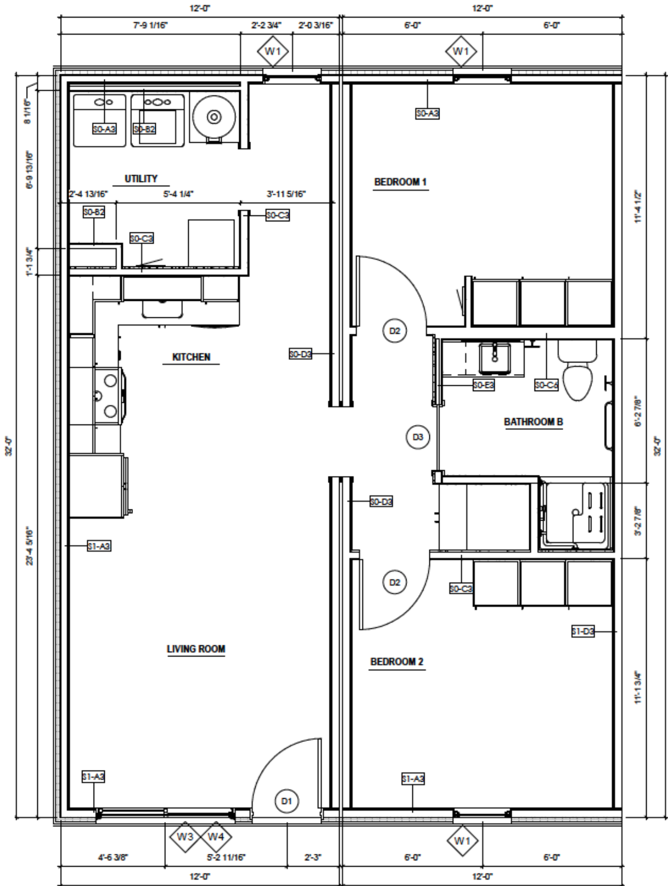
BUILDING 2, LEVEL 2, UNIT 1 FLOOR PLAN 3/8" = 1'-0"
