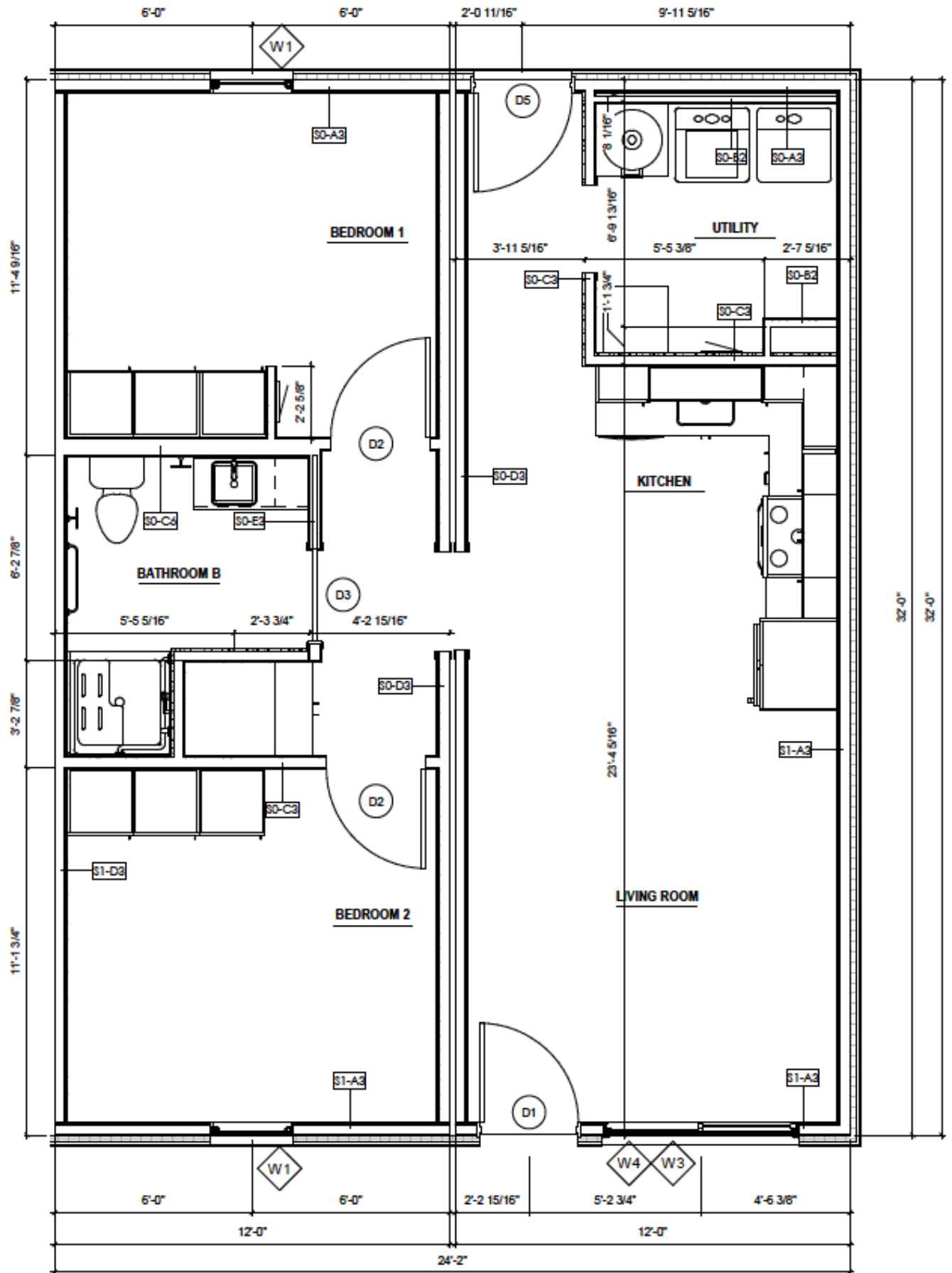
BUILDING 2, LEVEL 1, UNIT 2 FLOOR PLAN 3/8" = 1'-0"
